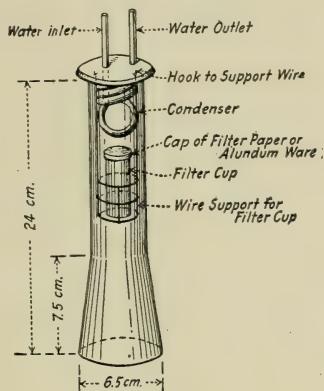
FIG. 190.—Cary-Curr Extraction Apparatus.
